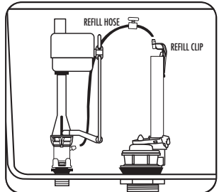
Correct set up of refill hose and refill clip to overflow pipe.
