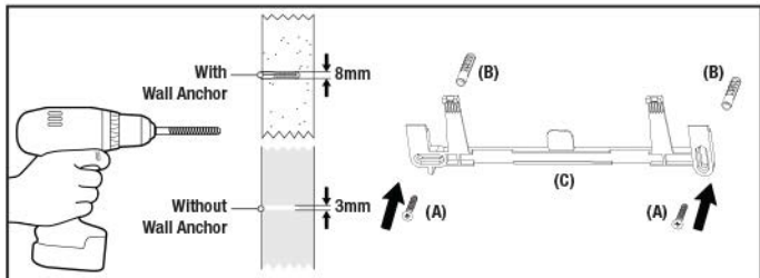
C) Wall Fixing Bracket
